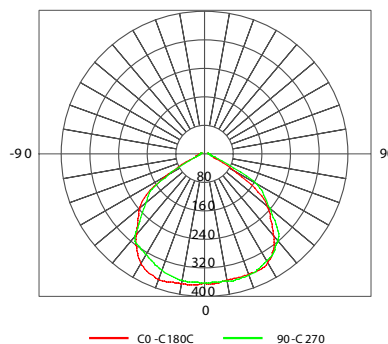
cd/1000 lm Curve
